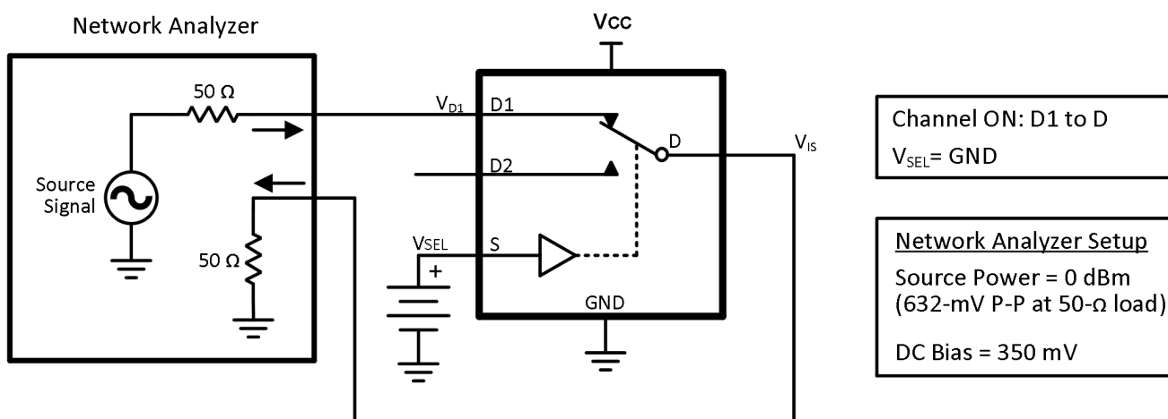
Figure 11. Bandwidth (BW)
