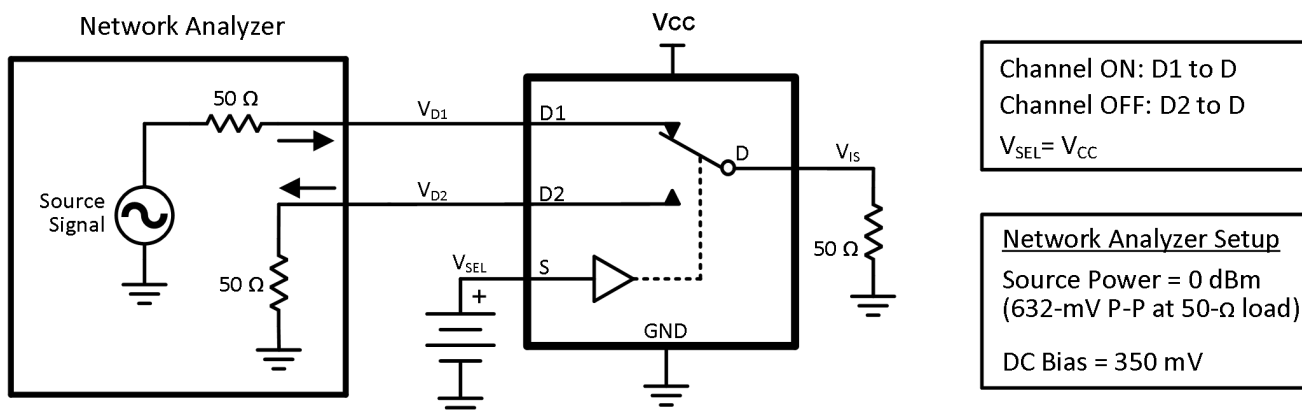
Figure 10. Crosstalk ( X_{TALK} )
