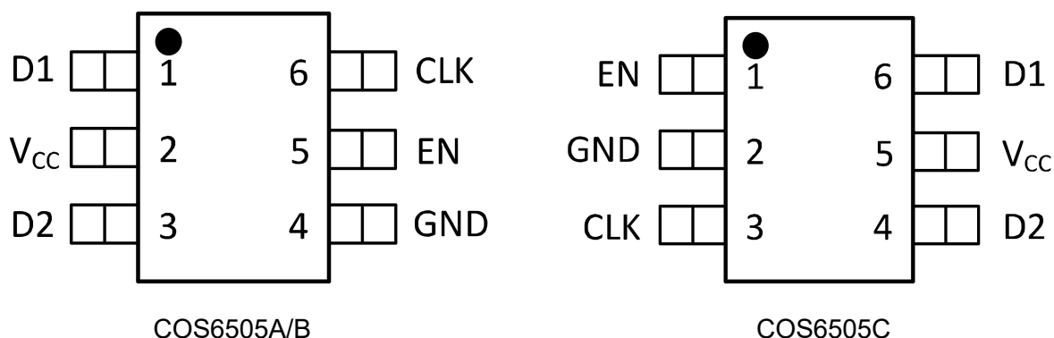
Figure 1 Pin Diagram
