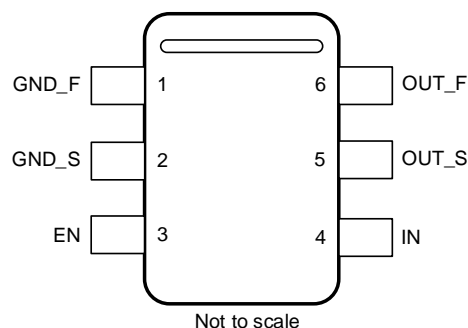
Figure 1. CI3433 6-Pin SOT-23 Top View
