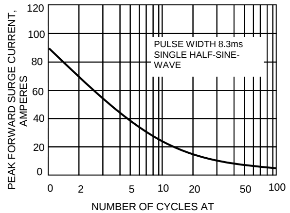
FIG.2-MAXIMUM NON-REPETITIVE SURGE
