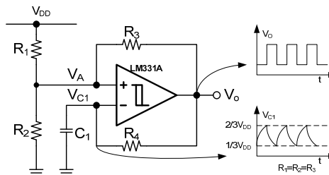
Figure 7. Relaxation Oscillator
