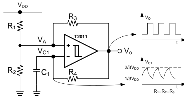
Figure 8. Relaxation Oscillator
