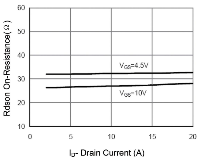
Figure 6 Drain-Source On-Resistance
