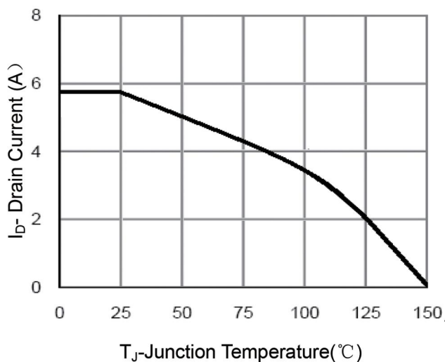
Figure 4 Drain Current
