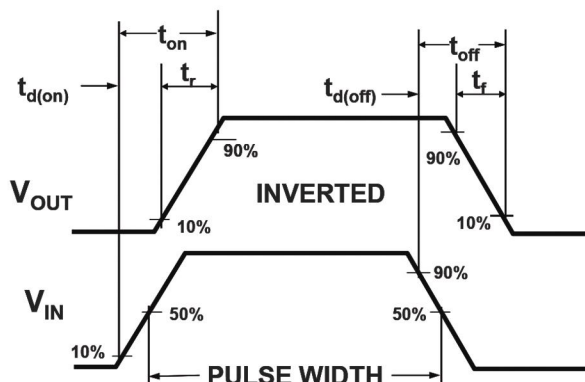
Figure 2: Switching Waveforms
